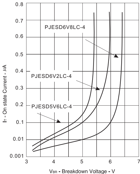
Figure 2.IT-VBR CHARACTERISTICS
