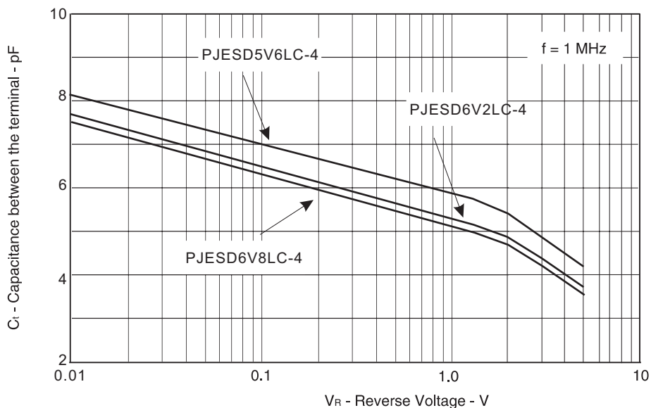
Figure 3.CT-VR CHARACTERISTICS
