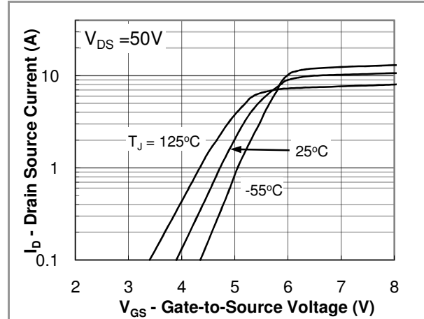
Fig.2 Transfer Characteristic
