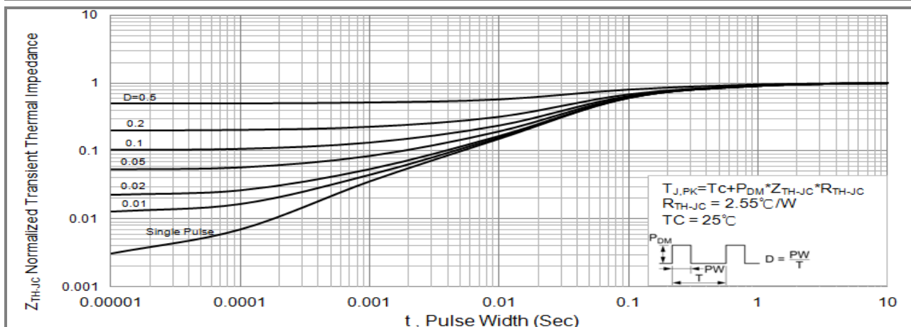
Fig.15 PJF8NA50 Normalized Transient Thermal Impedance vs. Pulse Width
