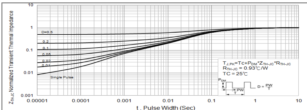
Fig.14 PJP8NA50 Normalized Transient Thermal Impedance vs. Pulse Width
