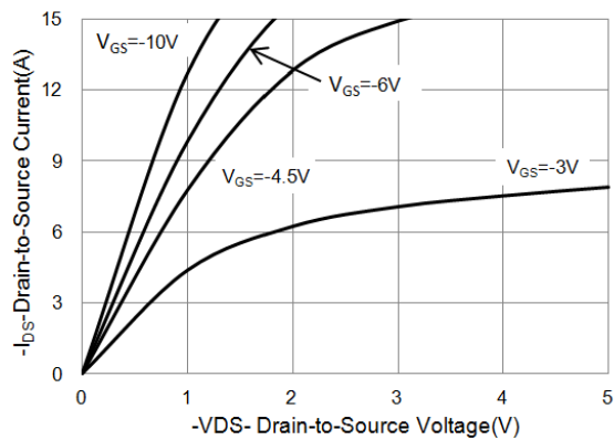
Fig.1 On-Region Characteristics
