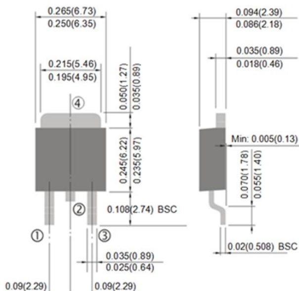
TO-252AA Dimension
