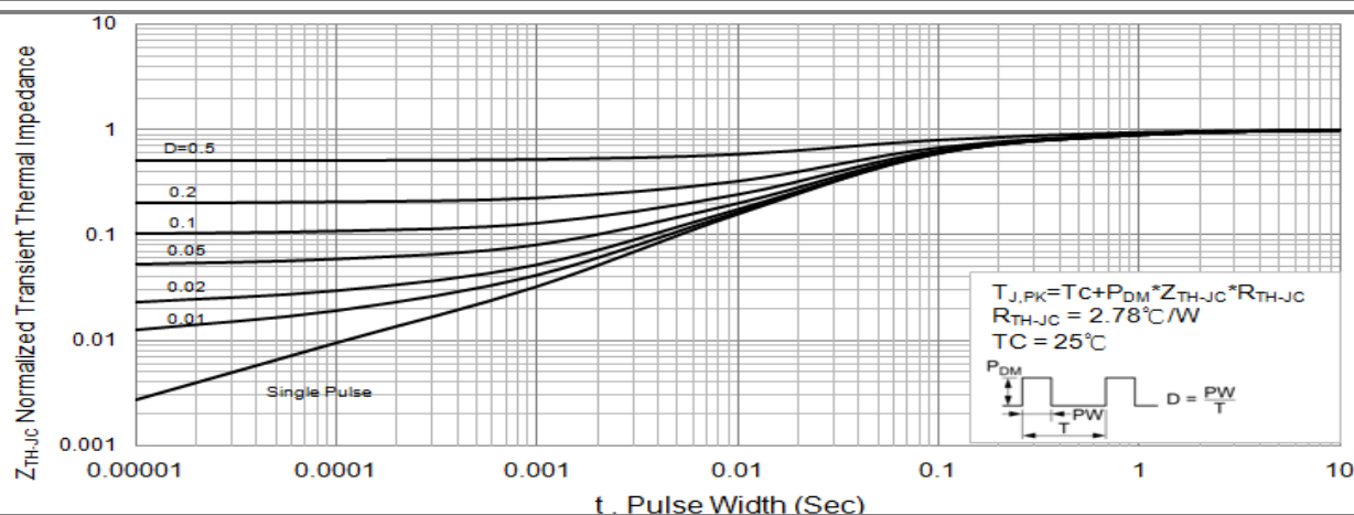
Fig.15 PJF6NA70 Normalized Transient Thermal Impedance vs. Pulse Width
