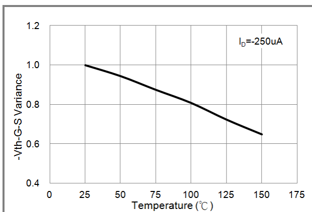
Fig.6 Threshold Voltage
