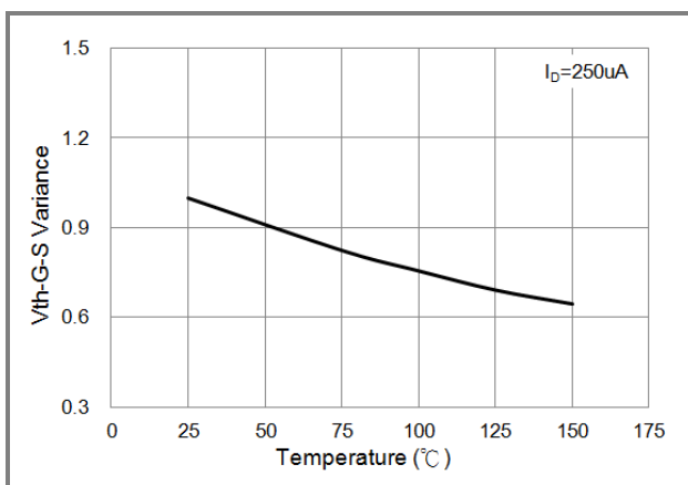
Fig.6 Threshold Voltage
