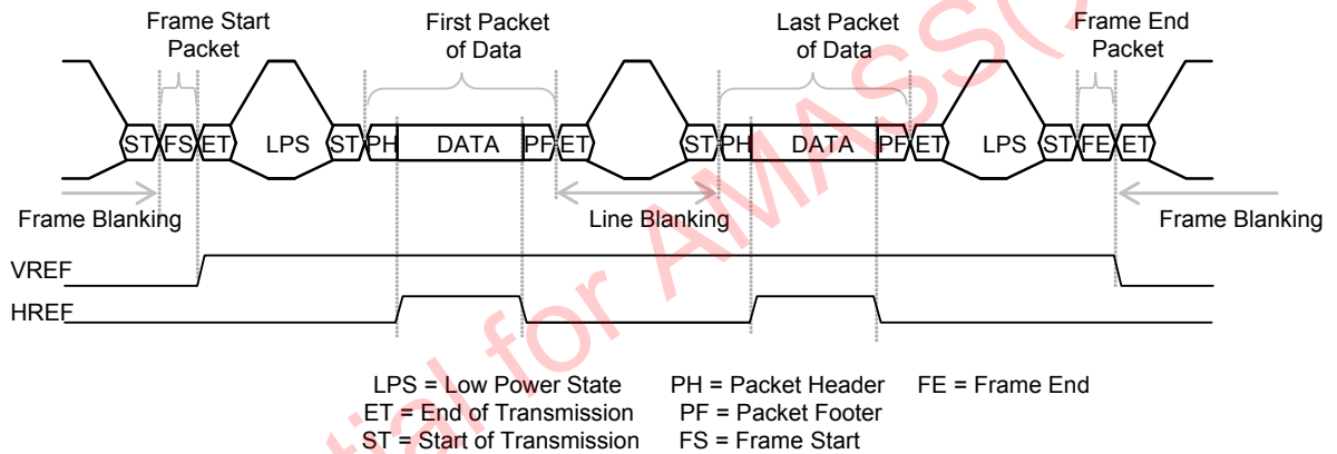
Figure 39 MIPI multiple packet
