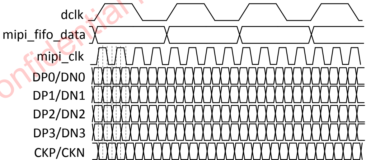
Figure 32 MIPI clock relations diagram
