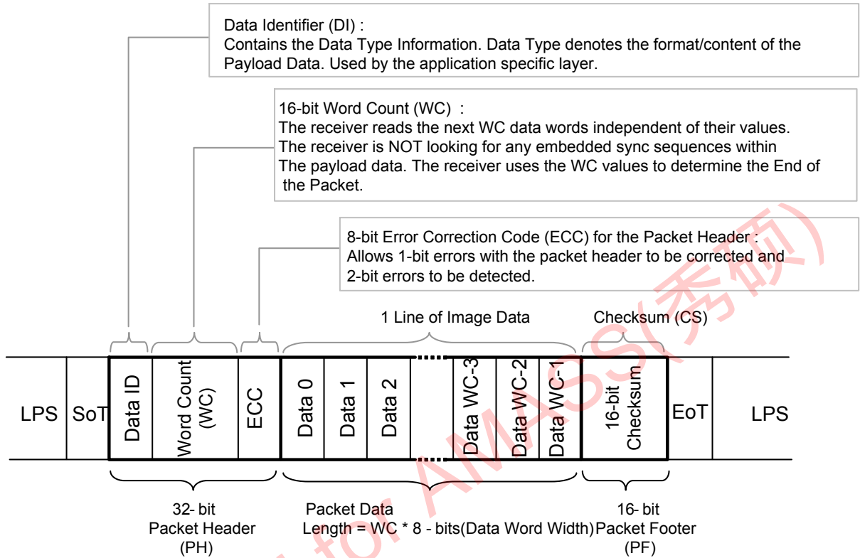
Figure 38 MIPI long packet structure
