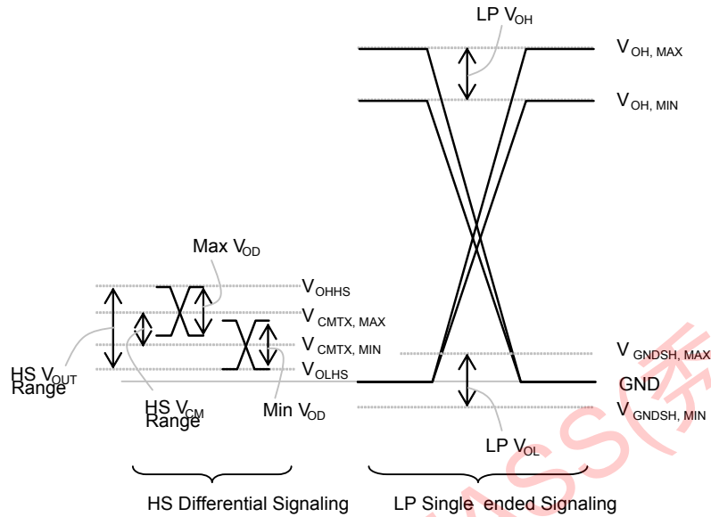
Figure 40 D-PHY signaling levels
