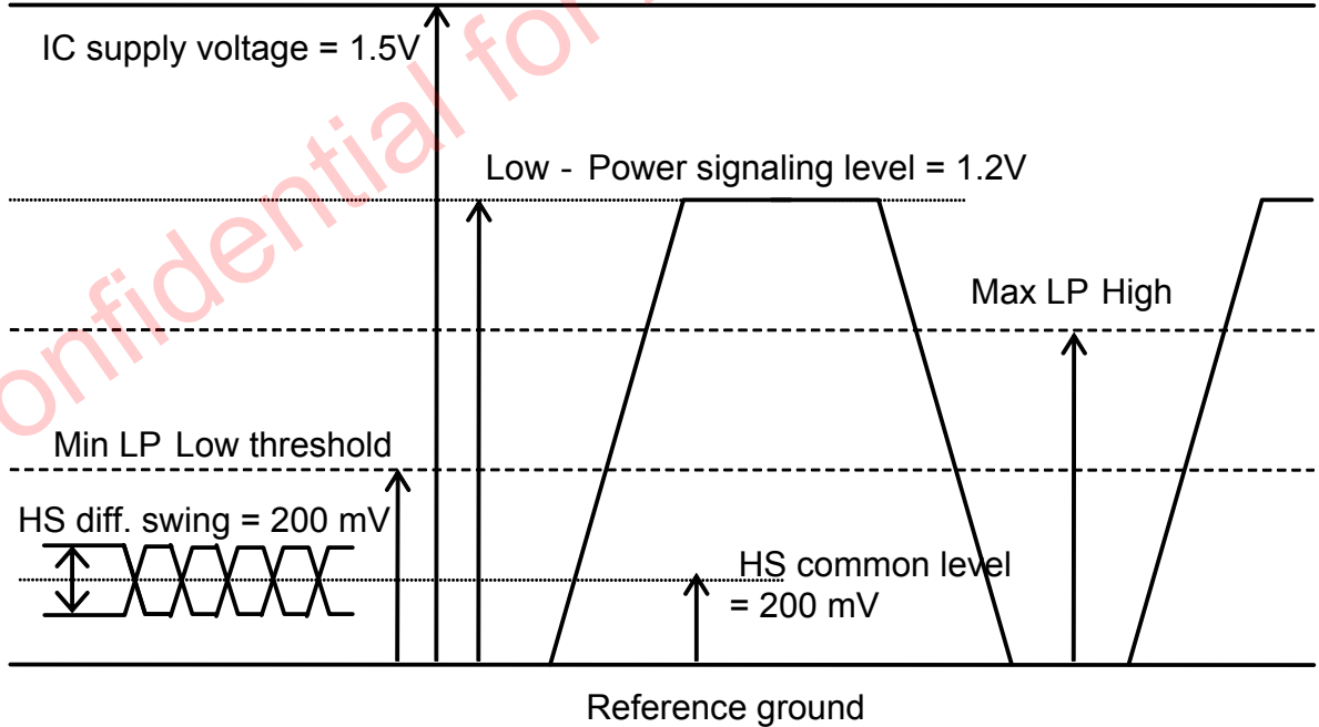
Figure 35 MIPI PAD levels
