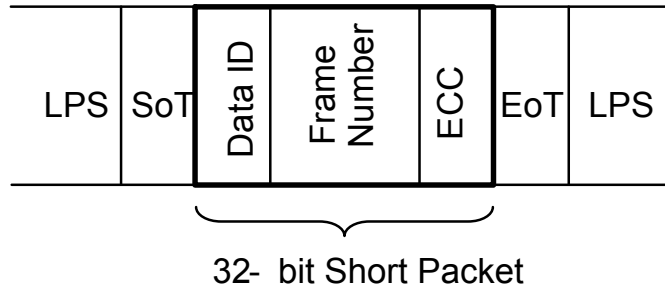
Figure 37 MIPI short packet structure
