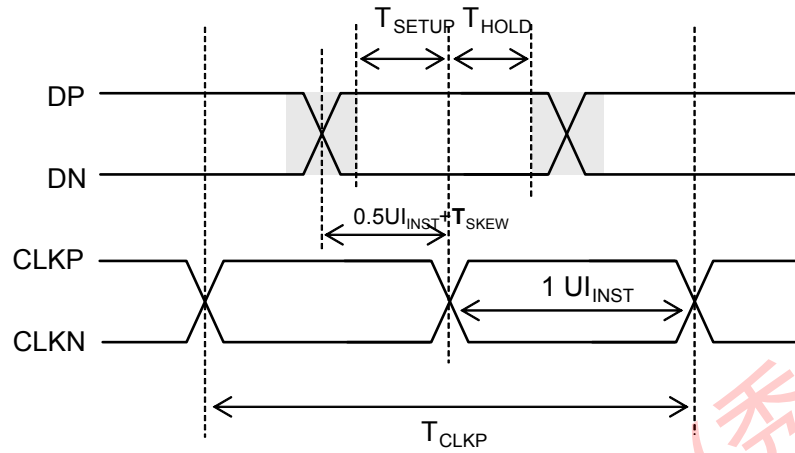
Figure 41 Data to clock timing
