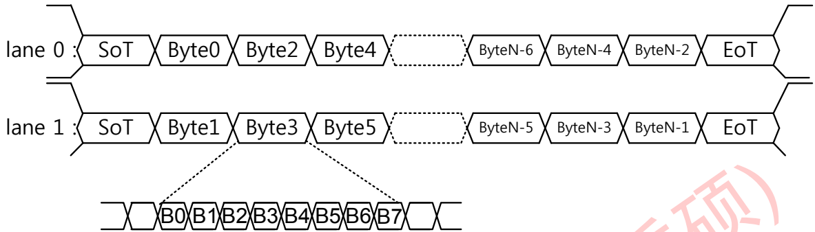
Figure 34 MIPI transmission order
