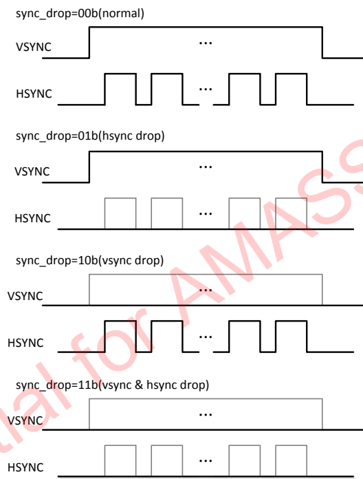
Figure 7 Sync drop
