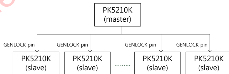
Figure 21 Genlock Sync configuration with another the PK5210K
