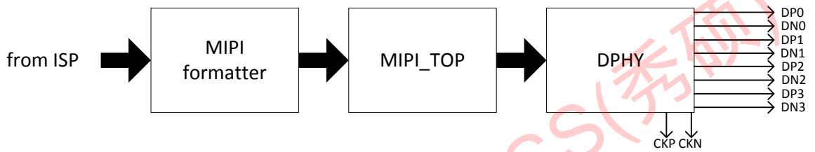
Figure 31 MIPI block diagram
