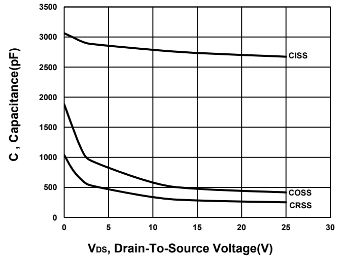
Capacitance Characteristic
