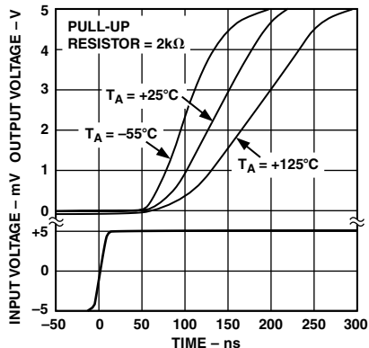
TPC 38. Comparator Response Time vs. Temperature
