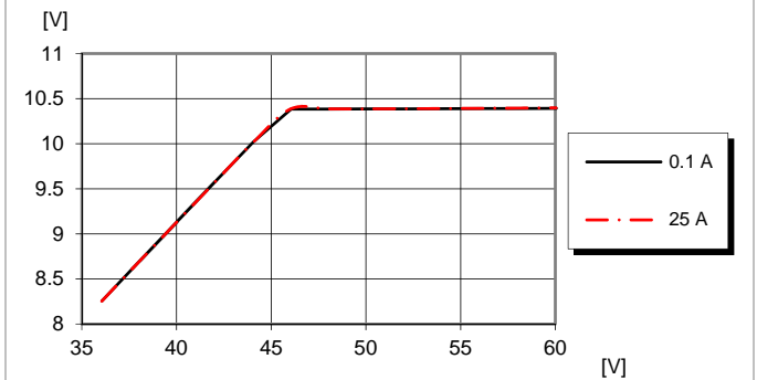
Output voltage vs. input voltage and load current at T_{P1} = +25^{\circ}\text{C} .
