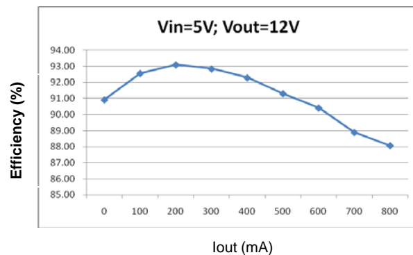
Figure 2. Efficiency Curve
