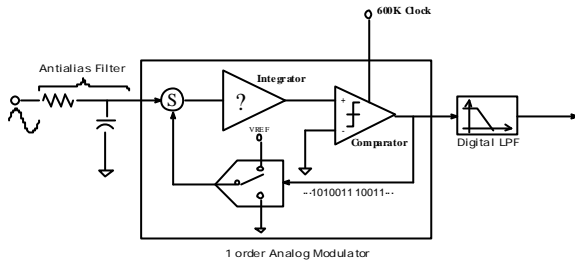
figure1 first order type ADC principle chart
