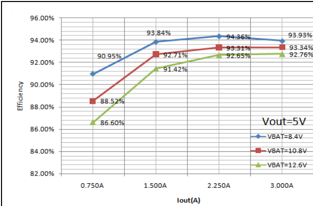
Fig. 3 Efficiency
