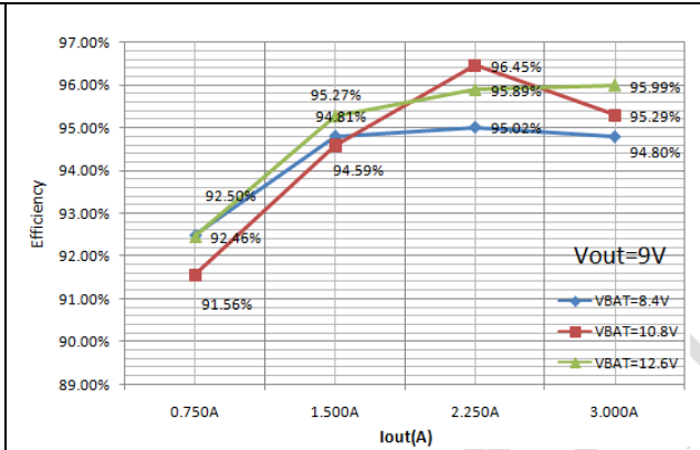
Fig. 4 Efficiency
