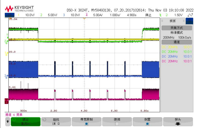
Fig.21 Steady State waveform Iout =3A
