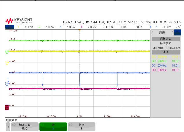
Fig.15 Start up waveform through EN, Iout =3A
