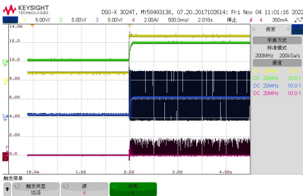
CH1:Vin CH2:Vout CH3:SW CH4:IL Vin=12V Vout=5V Fig.8 Start up waveform through Vin, Iout =0A
