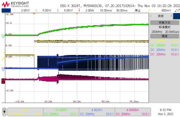
CH1:EN CH2:Vout CH3:SW CH4:IL Vin=5V Vout=5V Fig.6 Start up waveform through EN, Iout =0A
