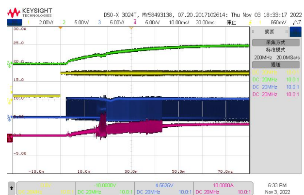
CH1:EN CH2:Vout CH3:SW CH4:IL Vin=5V Vout=5V Fig.7 Start up waveform through EN, Iout =3A
