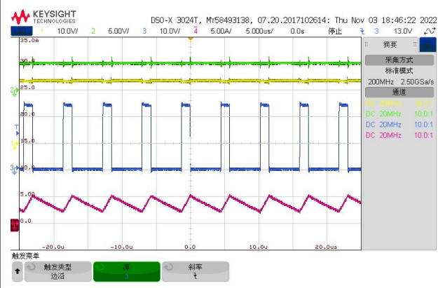
Fig.19 Steady State waveform Iout =3A
