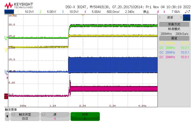
CH1:Vin CH2:Vout CH3:SW CH4:IL Vin=12V Vout=5V Fig.9 Start up waveform through Vin, Iout =3A
