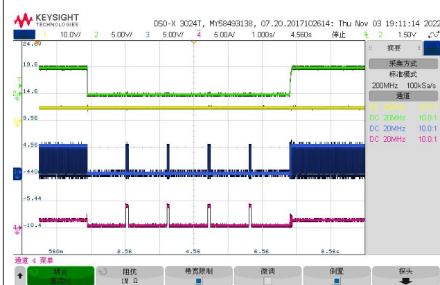
Fig.20 Steady State waveform Iout =0A
