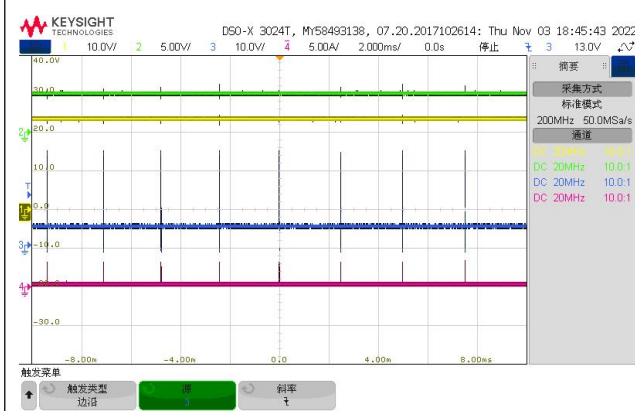
Fig.18 Steady State waveform Iout =0A
