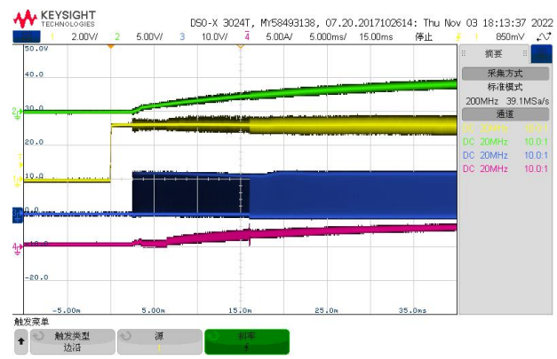
CH1:EN CH2:Vout CH3:SW CH4:IL Vin=12V Vout=5V Fig.11 Start up waveform through EN, Iout =3A
