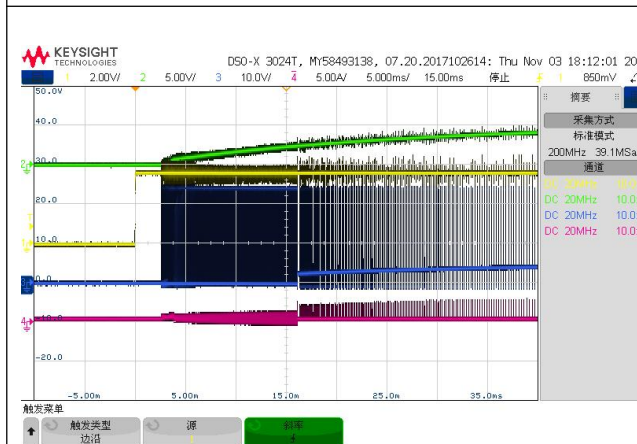
Fig.12 Start up waveform through Vin, Iout =0A
