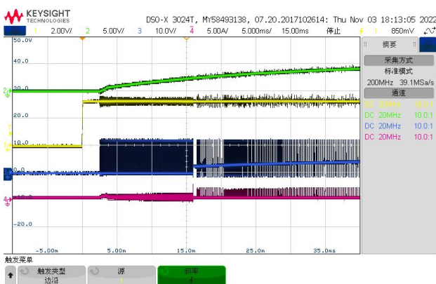
CH1:EN CH2:Vout CH3:SW CH4:IL Vin=12V Vout=5V Fig.10 Start up waveform through EN, Iout =0A
