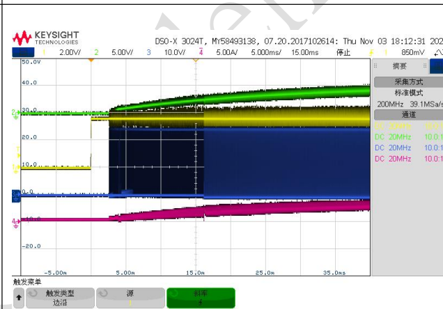
Fig.13 Start up waveform through Vin, Iout =3A
