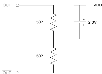
LVPECL Levels Test Circuit
