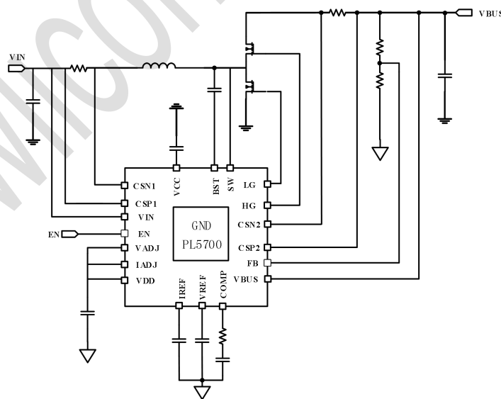
Fig. 1 Application Schematic
