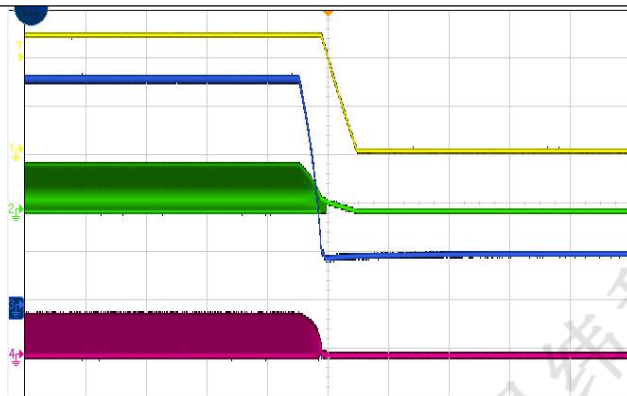
Fig. 15 Power Down Waveform, Iout =6A
