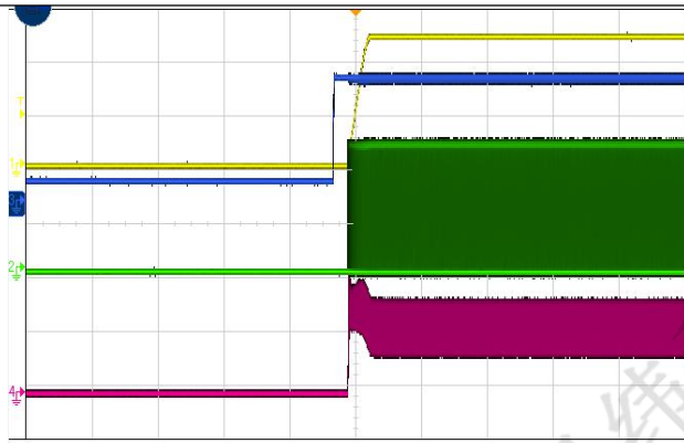
Fig. 9 Power Up Waveform, Iout =1A
