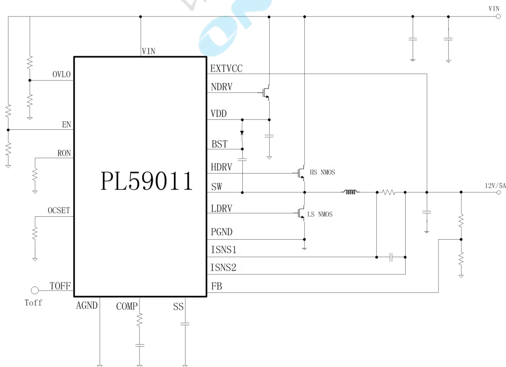
Fig. 1 Application Schematic
