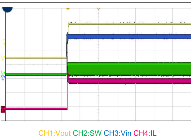
Fig. 6 Power Up Waveform, Iout =2A
