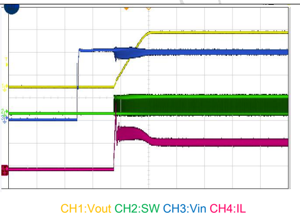
Fig. 5 Power Up Waveform, Iout =0A
