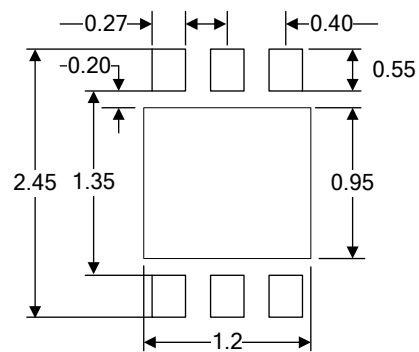
Recommended Land Pattern (MM)
