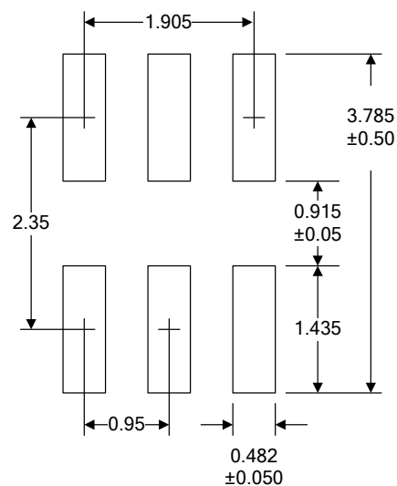
Recommended Land Pattern (MM)
