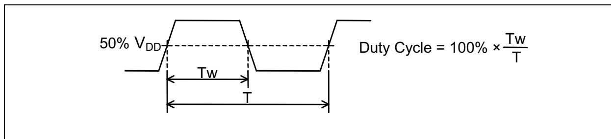
FIGURE 4-3: Duty Cycle.
