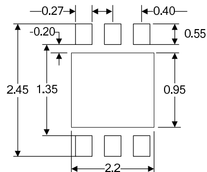
Recommended Land Pattern (MM)
