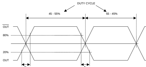
PECL Transition Time Waveform
