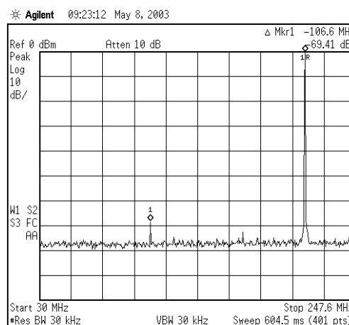
Figure 4: Spectrum Analysis at 212.5MHz Analog Frequency Multiplier (2x), with sub-harmonics below -69dBc
