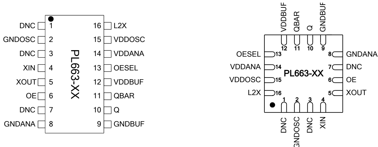
2x AFM Package Pin Out
