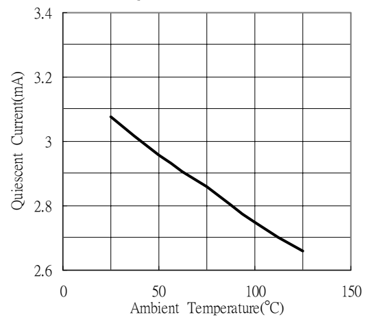
Quiescent Current
