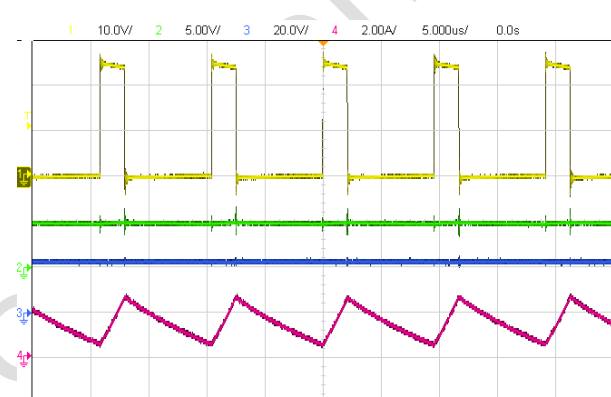
Vin = 24V, Vout = 5V Ch1: SW Ch2: VOUT Ch3: VIN Ch4: IL Fig. 13 Steady state waveform, Iout = 1A
