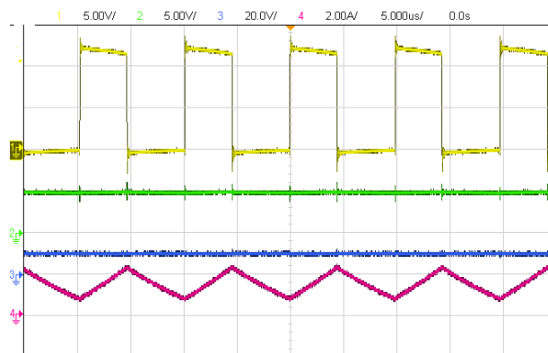
Vin = 12V, Vout = 5V Ch1: SW Ch2: VOUT Ch3: VIN Ch4: IL Fig. 11 Steady state waveform, Iout = 1A
