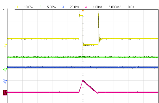
Vin = 24V, Vout = 5V Ch1: SW Ch2: VOUT Ch3: VIN Ch4: IL Fig. 12 Steady state waveform, Iout = 0A
