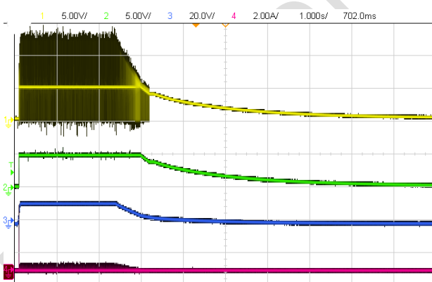
Vin = 12V, Vout = 5V Ch1: SW Ch2: VOUT Ch3: VIN Ch4: IL Fig. 14 Shutdown waveform, Iout = 0A
