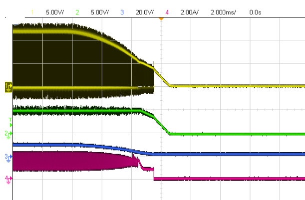
Vin = 12V, Vout = 5V Ch1: SW Ch2: VOUT Ch3: VIN Ch4: IL Fig. 15 Shutdown waveform, Iout = 1A
