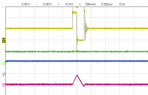
Vin = 12V, Vout = 5V Ch1: SW Ch2: VOUT Ch3: VIN Ch4: IL Fig. 10 Steady state waveform, Iout = 0A
