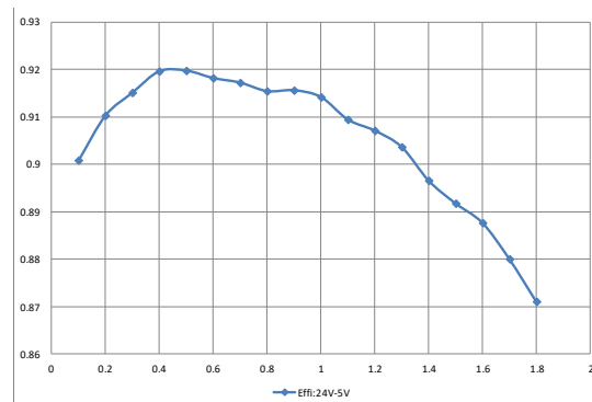
Fig. 5 Efficiency
