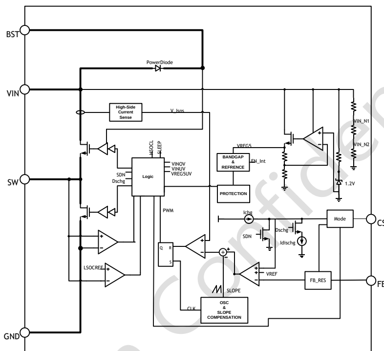
Fig.16 PL8310E Diagram
