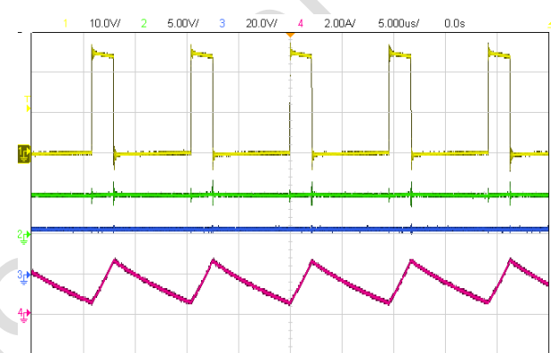
Fig. 11 Steady state waveform, Iout = 1A
