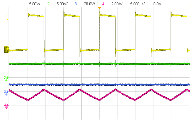
Fig. 11 Steady state waveform, Iout = 1A
