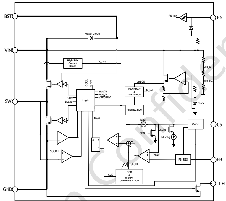
Fig.16 PL8312 Diagram
