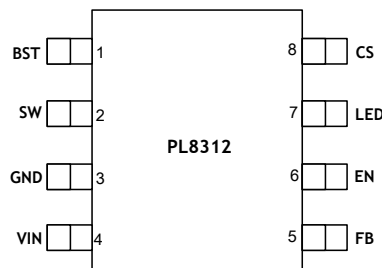
Fig3. SOP-8 Package
