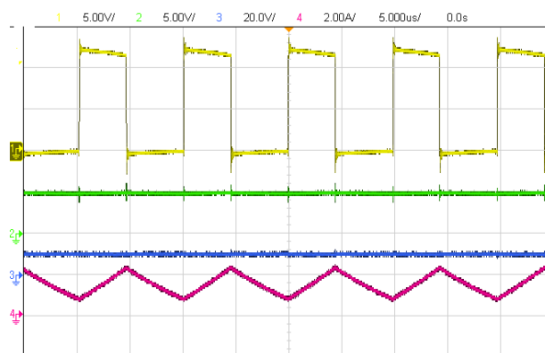
Fig. 11 Steady state waveform, Iout = 1A
