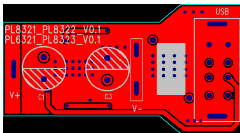
Fig. 25 Top layer layout for car charger
