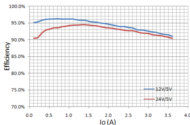
Fig. 2 Efficiency curve
