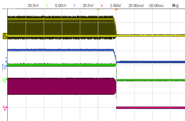
Fig. 14 Shutdown waveform, Iout = 3A
