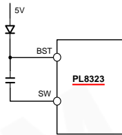
Fig. 20 External Bootstrap Diode
