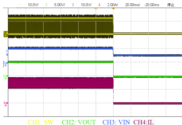
Fig. 10 Shutdown waveform, Iout = 3A
