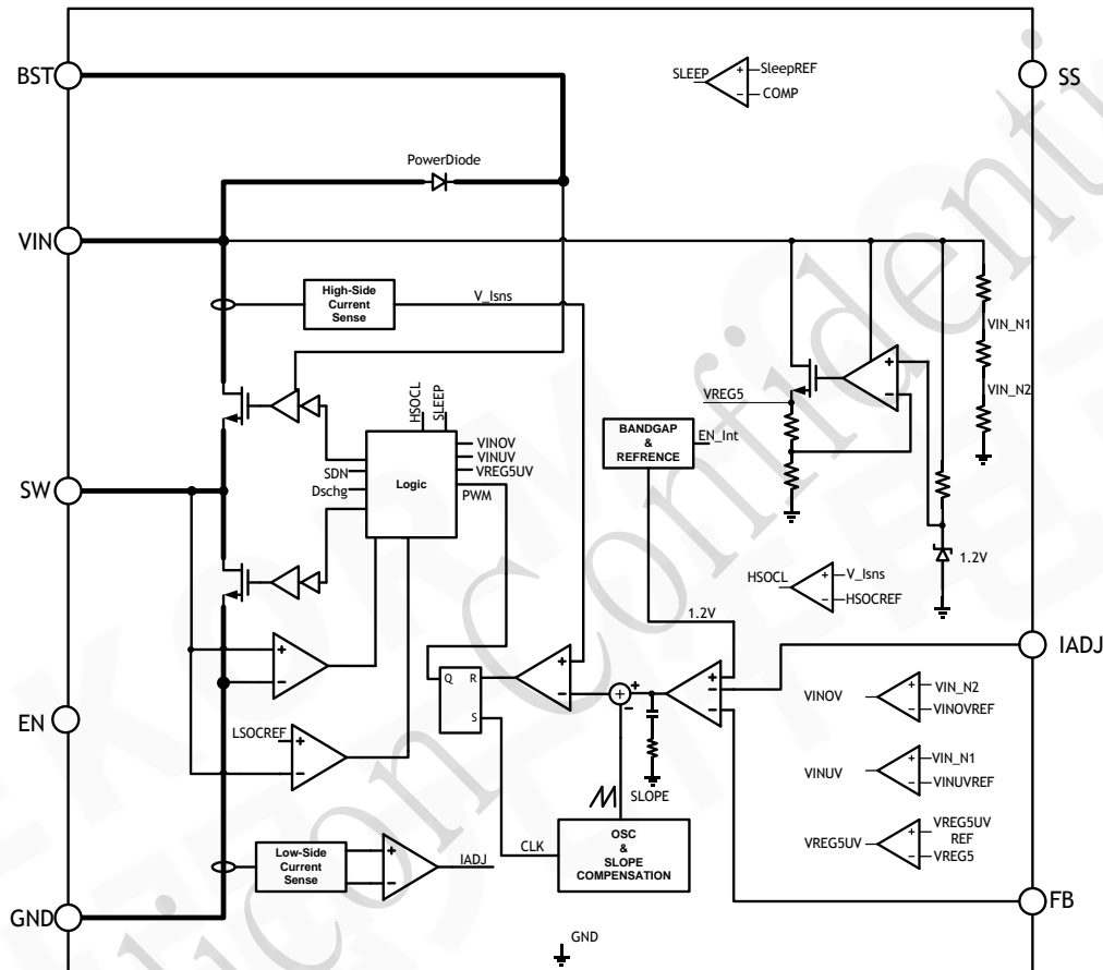
Fig.19 PL8323 Diagram
