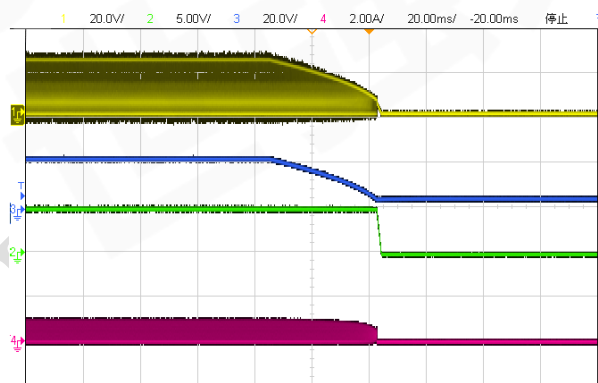
Fig. 13 Shut down waveform, Iout = 0.3A
