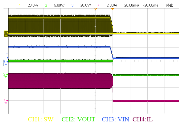
Fig. 14 Shutdown waveform, Iout = 2.5A
