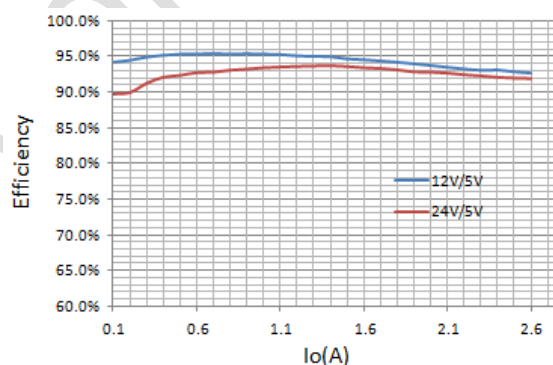
Fig. 2 Efficiency curve
