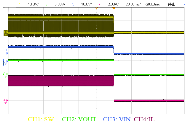
Fig. 10 Shutdown waveform, Iout = 2.5A
