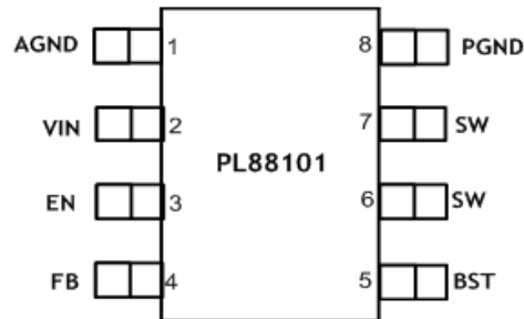
Fig.4 SOP8 Package
