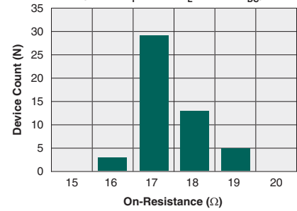
Typical On-Resistance Distribution (N=50, I_F=5mA , I_L=150mA_{DC} )
