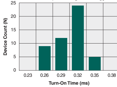
Typical Turn-On Time (N=50, I_F=5mA , I_L=100mA_{DC} )
