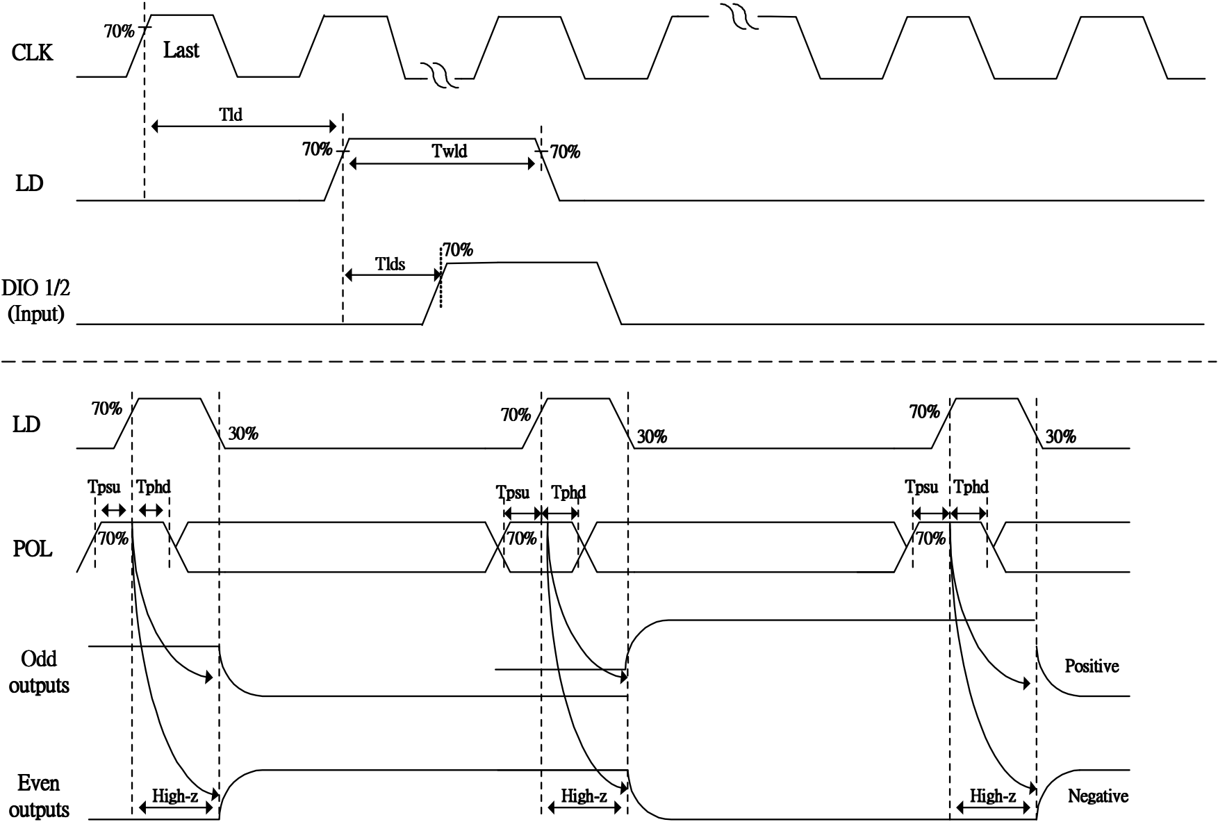
Fig. 11-2 Horizontal timing(2)
