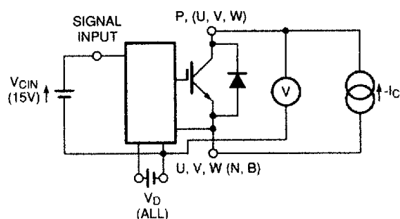
Figure 3 V_{EC} Test
