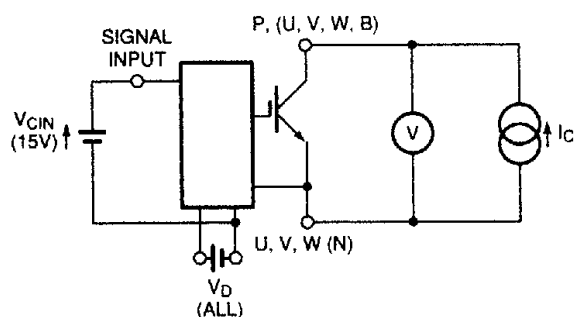
Figure 1 V_{CES} Test
