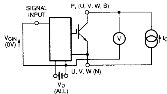
Figure 2 V_{CE(SAT)} Test
