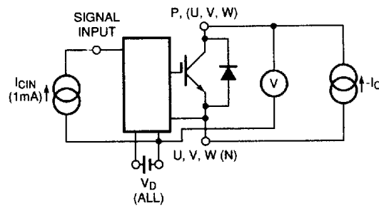
Figure 3 V_{EC} Test
