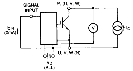
Figure 2 V_{CE(SAT)} Test
