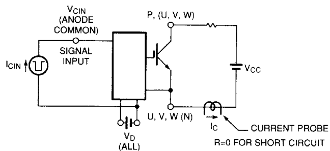
Figure 7 Over Current and Short Circuit Test
