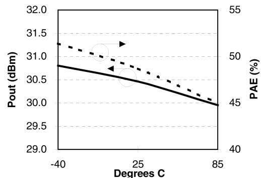
Output Power and Efficiency vs. Temperature
