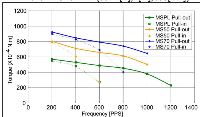
PM42L-048 BI-CHOPPER (at 24[V],7[Ω],600[mA])
