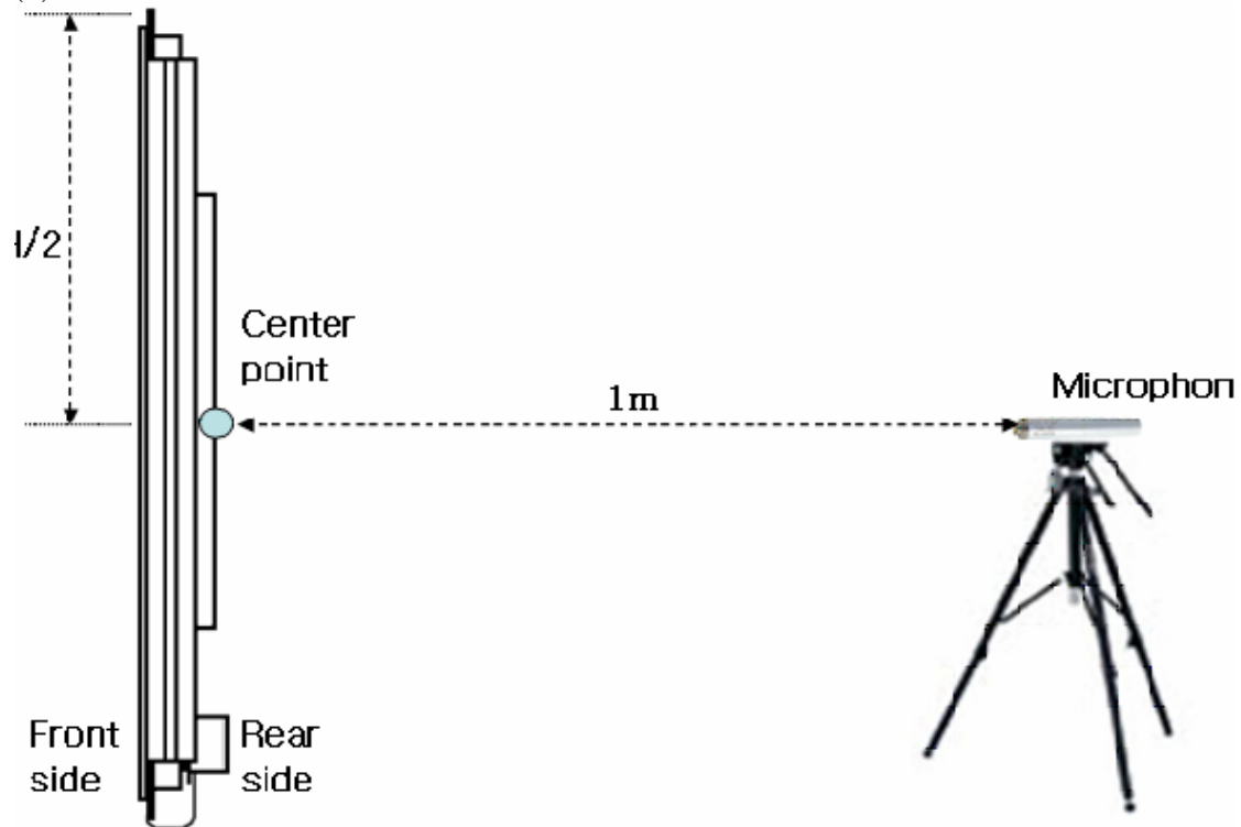
Figure 14 - Measuring layout
