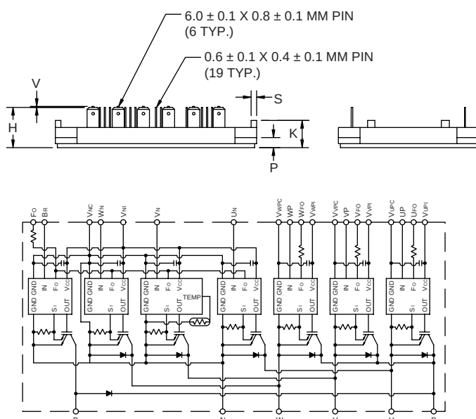
Outline Drawing and Circuit Diagram
