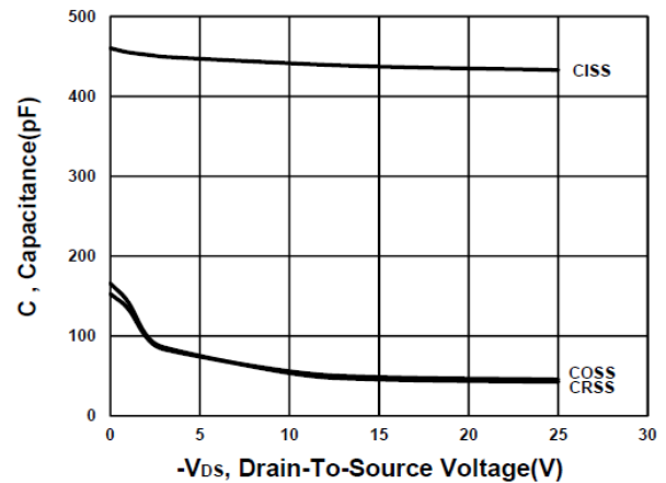
Capacitance Characteristic
