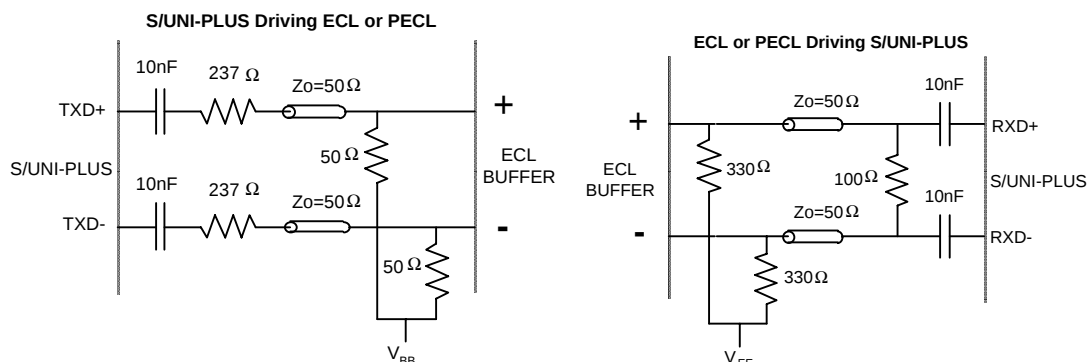
Figure 10 - Interfacing S/UNI-PLUS to ECL or PECL
