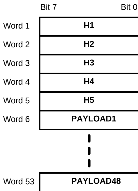
Figure 16 - 8-bit Wide, 53 Word Structure
