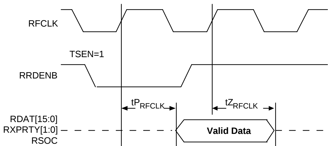
Figure 46 - Drop Side Receive Interface Timing, TSEN = 1
