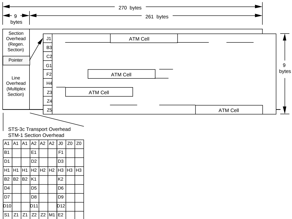
Figure 14 - STS-3c (STM-1) Mapping
