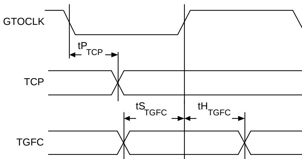
Figure 44 - Transmit GFC Access Timing
