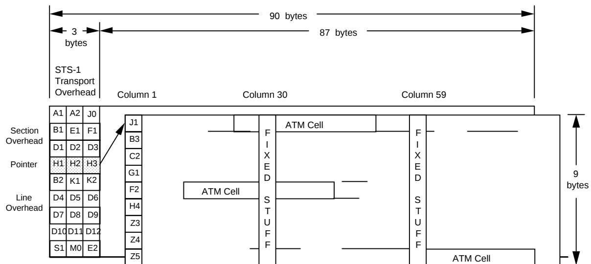
Figure 13 - STS-1 Mapping
