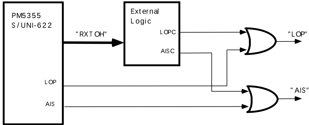
Figure 8 - ITU G.783 Concatenation Indicator Implementation
