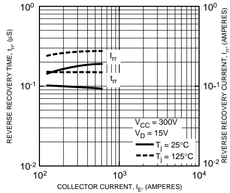
FWDI REVERSE RECOVERY CURRENT VS. COLLECTOR CURRENT (TYPICAL)
