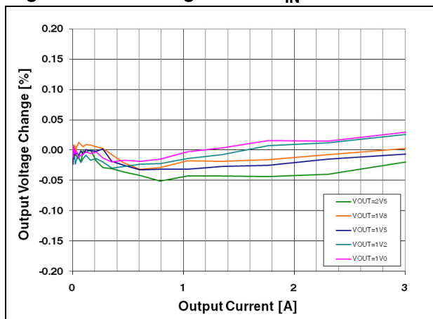
Figure 6. Load regulation - V_{IN} = 3.3\text{ V}
