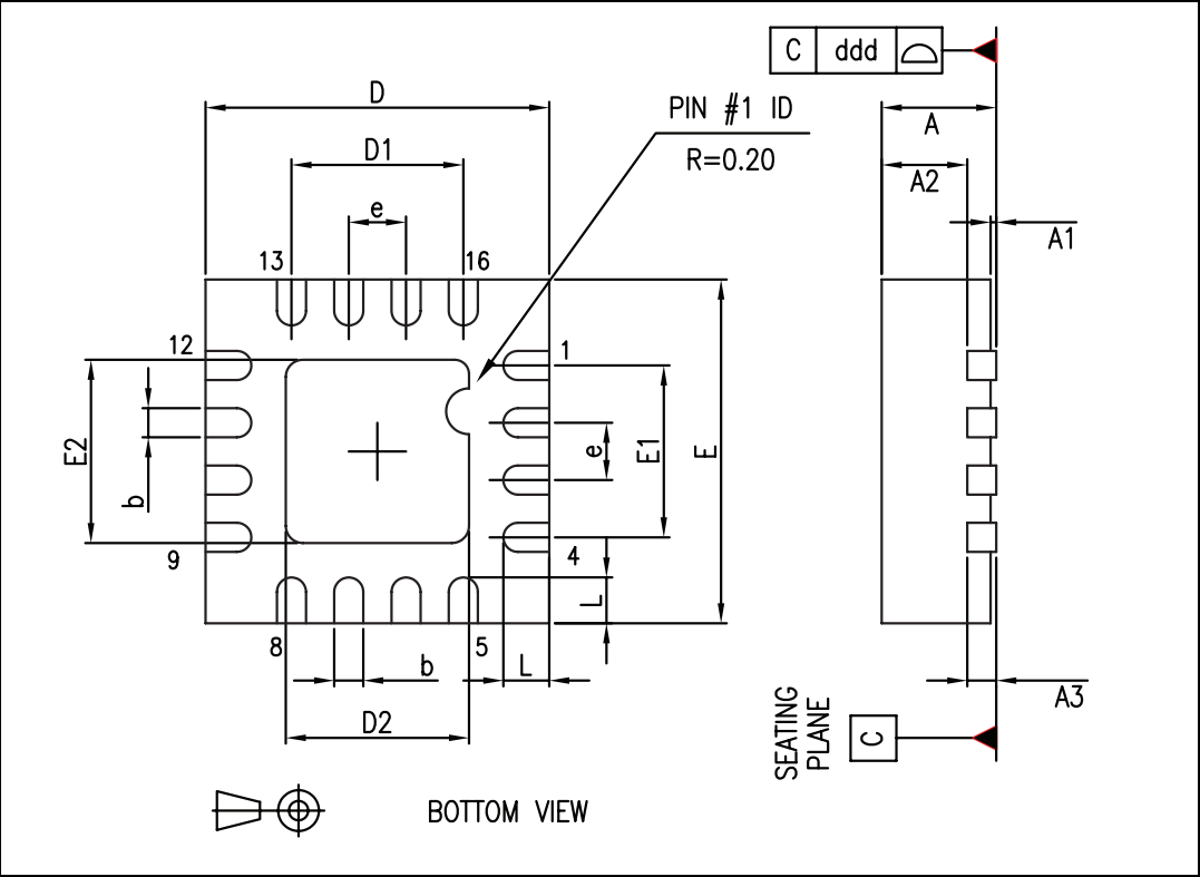
Figure 16. Package dimensions
