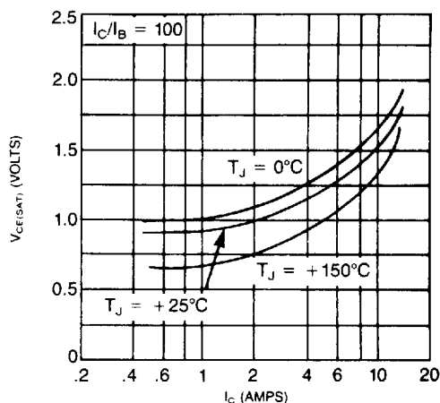
V_{CE(SAT)} VS COLLECTOR CURRENT
