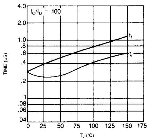
DYNAMIC CHARACTERISTICS VS JUNCTION TEMPERATURE
