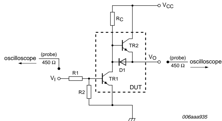
Fig 17. Test circuit for switching times
