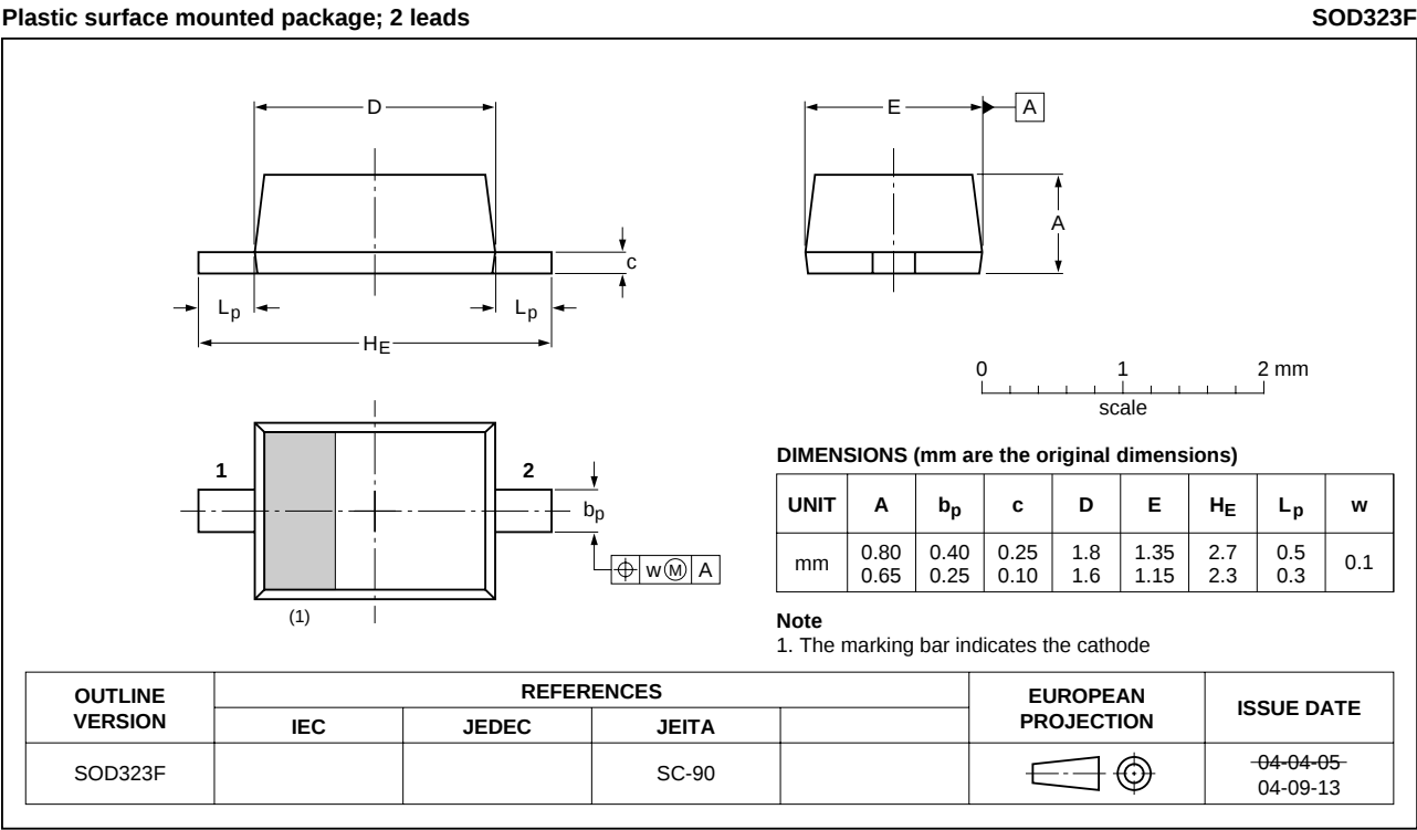
Fig 4. Package outline SOD323F (SC-90)
