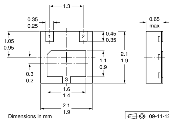
Fig 15. Package outline SOT1061
