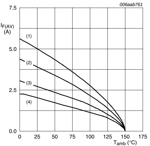
FR4 PCB, mounting pad for cathode 1\text{ cm}^2 T_j = 150^\circ\text{C} (1) \delta = 1 ; DC (2) \delta = 0.5 ; f = 20 kHz (3) \delta = 0.2 ; f = 20 kHz (4) \delta = 0.1 ; f = 20 kHz
