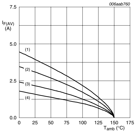
FR4 PCB, standard footprint T_j = 150^\circ\text{C} (1) \delta = 1 ; DC (2) \delta = 0.5 ; f = 20 kHz (3) \delta = 0.2 ; f = 20 kHz (4) \delta = 0.1 ; f = 20 kHz
