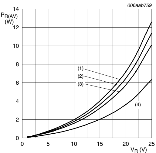
T_j = 125^\circ\text{C} (1) \delta = 1 (2) \delta = 0.9 (3) \delta = 0.8 (4) \delta = 0.5
