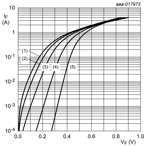
pulsed condition (1) T j = 150 °C (2) T j = 125 °C (3) T j = 85 °C (4) T j = 25 °C (5) T j = -40 °C
