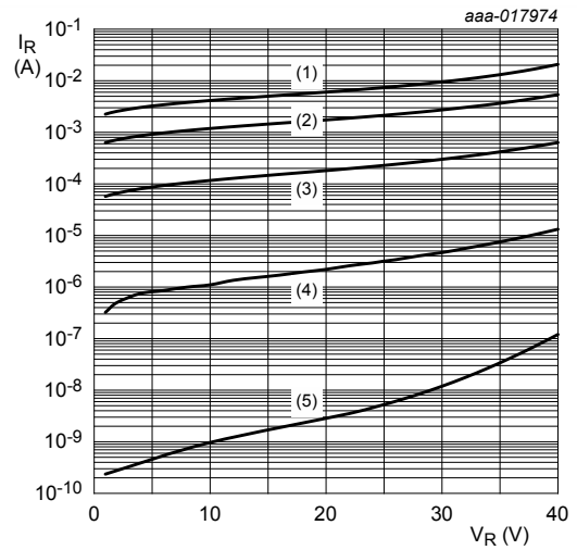
pulsed condition (1) T j = 150 °C (2) T j = 125 °C (3) T j = 85 °C (4) T j = 25 °C (5) T j = -40 °C
