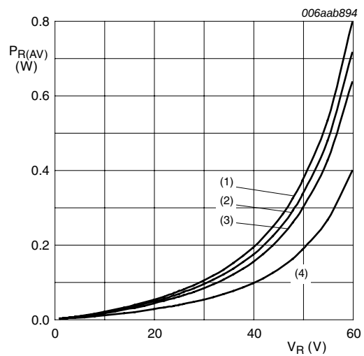
T_j = 125^\circ\text{C} (1) \delta = 1 (2) \delta = 0.9 (3) \delta = 0.8 (4) \delta = 0.5
