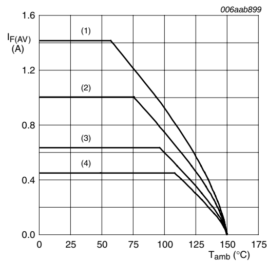
FR4 PCB, standard footprint T_j = 150^\circ\text{C} (1) \delta = 1 ; DC (2) \delta = 0.5 ; f = 20\text{ kHz} (3) \delta = 0.2 ; f = 20\text{ kHz} (4) \delta = 0.1 ; f = 20\text{ kHz}
