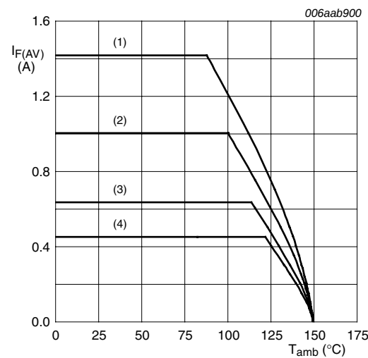
FR4 PCB, mounting pad for cathode 1\text{ cm}^2 T_j = 150^\circ\text{C} (1) \delta = 1 ; DC (2) \delta = 0.5 ; f = 20\text{ kHz} (3) \delta = 0.2 ; f = 20\text{ kHz} (4) \delta = 0.1 ; f = 20\text{ kHz}
